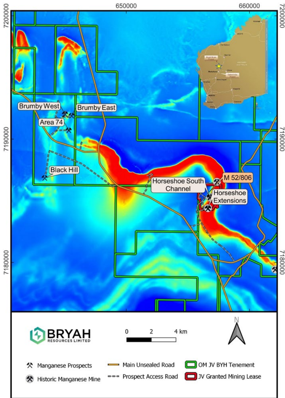
Figure 2 Location of Mn JV prospects with Mineral Resource on Aeromagnetics TMI RTP image
